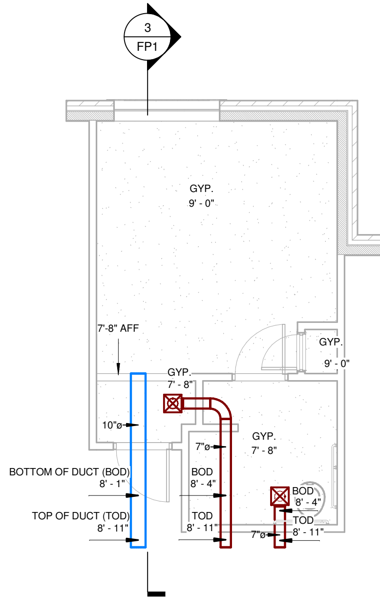
REFLECTED CEILING PLAN SCALE: 3/16" = 1'-0" NORTH
