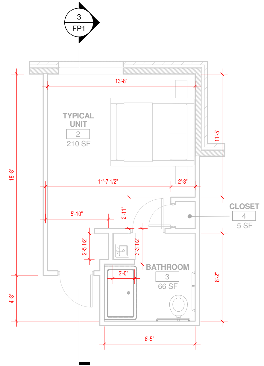
FLOOR PLAN SCALE: 3/16" = 1'-0" NORTH
